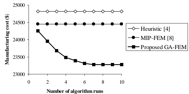
Fig. 2. Comparative results for an 1600 kVA transformer design.
